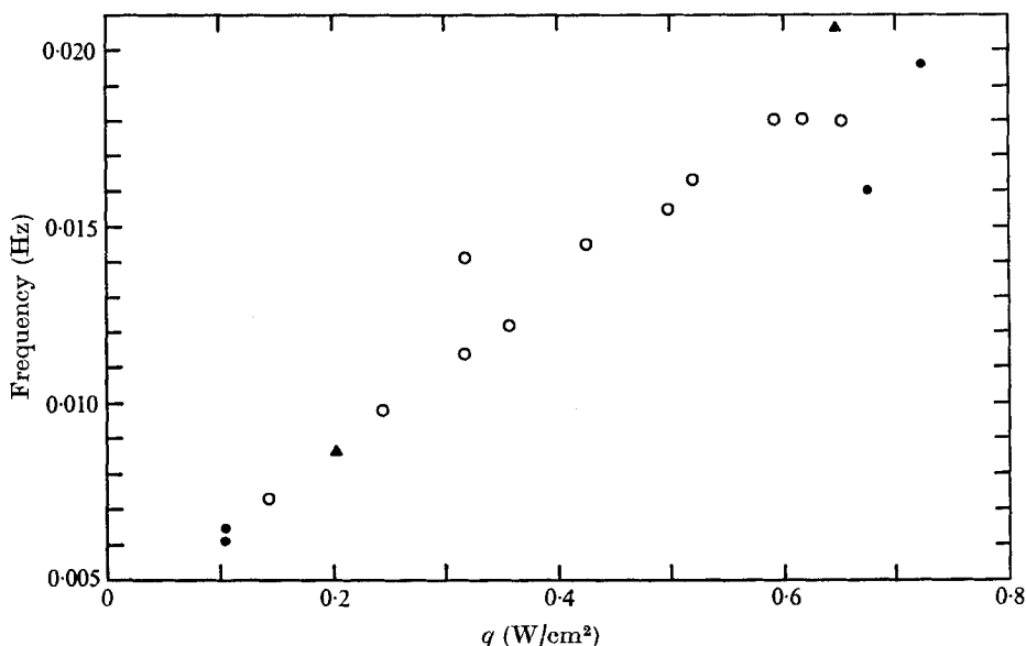
FIGURE 10. Experimentally observed frequency of oscillation as a function of imposed heat flux and comparison with analytically predicted conditions at the two neutral-stability points. Experiment: \circ , unstable; \bullet , neutrally stable. Analytical prediction: \blacktriangle , neutrally stable.
